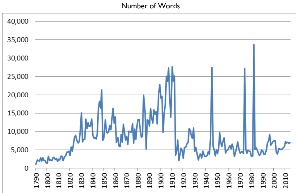
Figure 1. Length of the State of the Union Addresses, 1790-2015
